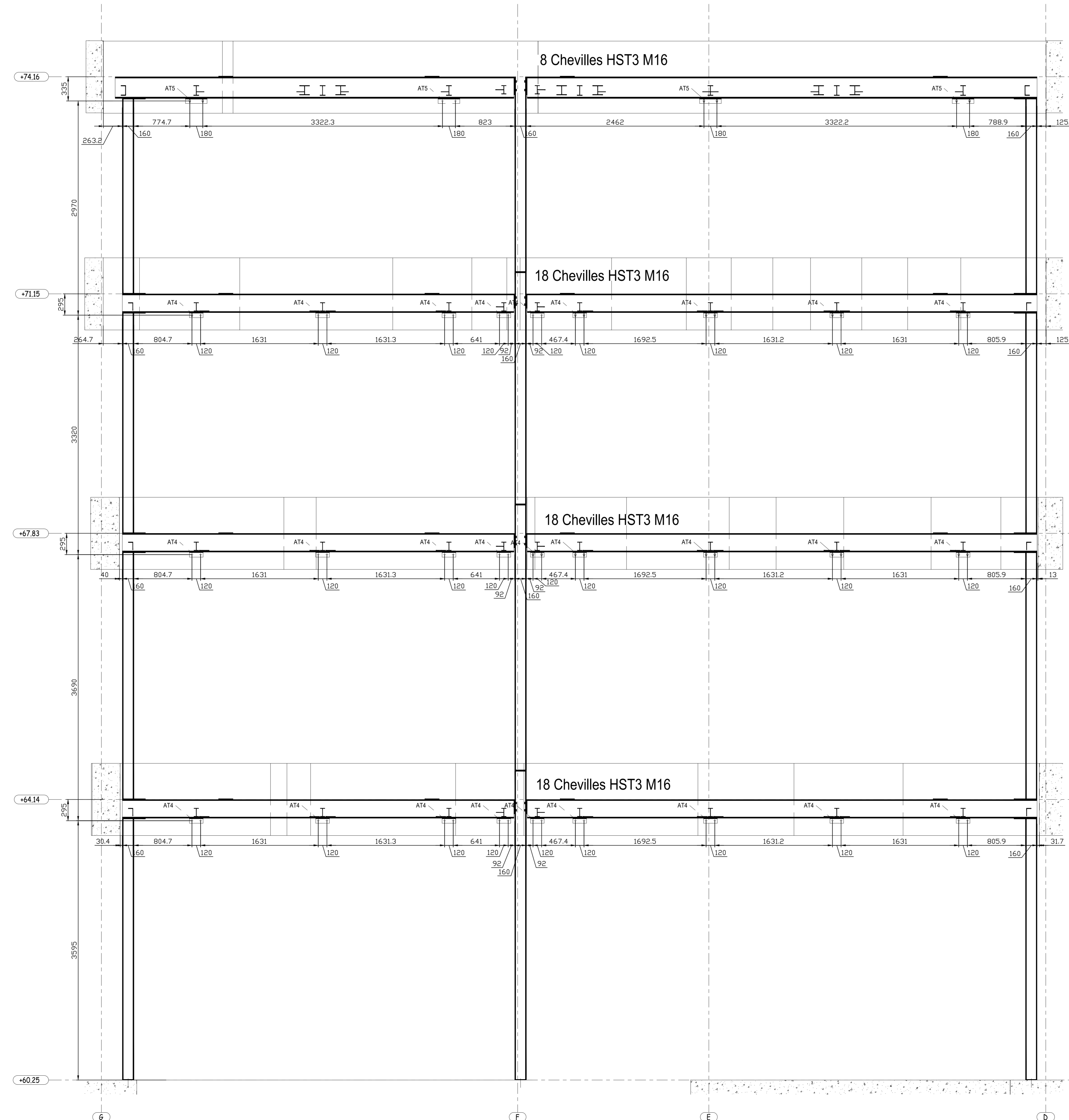
ELEVATION CHEVILLAGE 1/25
